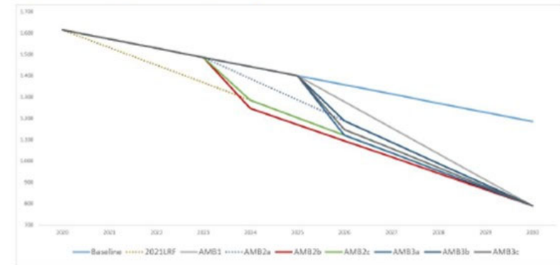
Figure 2: ETS cap under the different options
